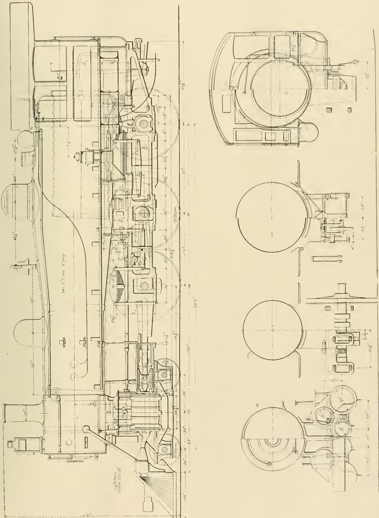
VAUCLAİN'S BALANCED FOUR-CYLINDER COMPOUND.
